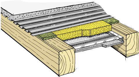
Type LWS-E1 brandwerendheid ≥ 60-90 minuten
